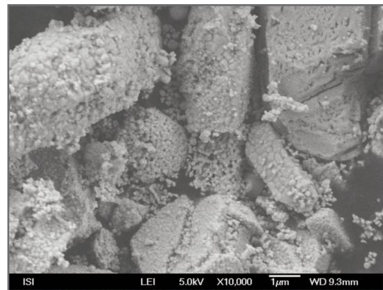
SEM Ceroxid HD R10S, x10.000
