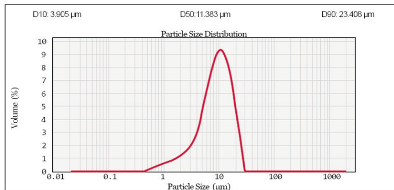
Ceroxid HD R10S PSD laser particle size distribution analyzer
